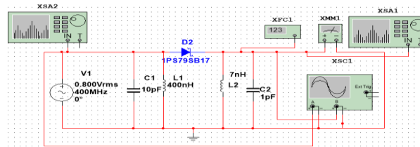
Fig. 5: Simulation Circuit Diagram of Frequency Doubling System Using Schottky Diode.
