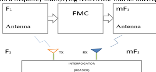
Fig. 1: Frequency Multiplying Reflectenna with Interrogator for IoT Application.
