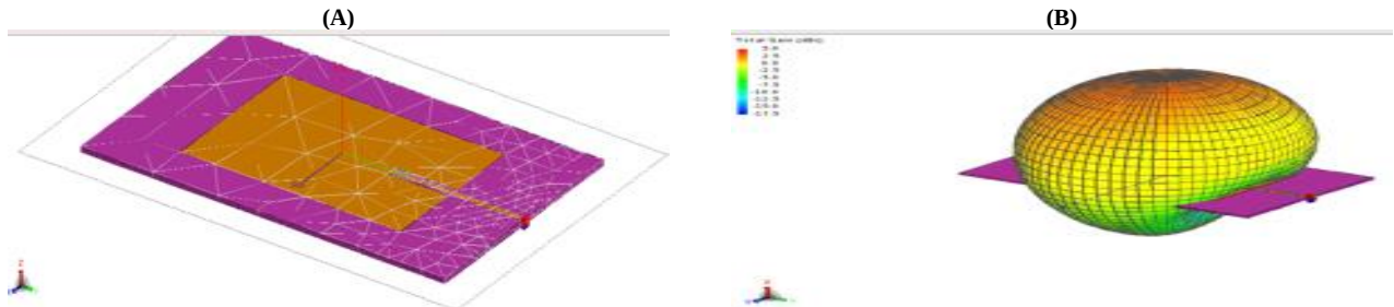
Fig. 8: A) Mf1 Microstrip Antenna, B) Simulated Radiation Pattern and Gain of Mf1 Microstrip Antenna for 866 Mhz.
