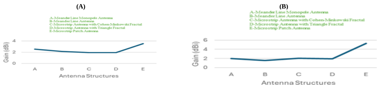
Fig. 9: Gain of Difference for Different Types of A) Microstrip Patch Antenna for 433 Mhz, B) Microstrip Patch Antenna for 866 Mhz.
