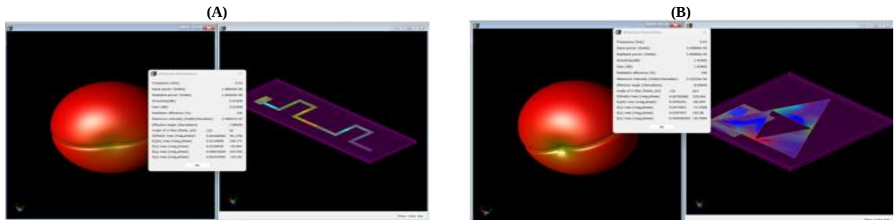
Fig. 7: 3-D Radiation Pattern with Gain In (DBI) and Current Distribution of A) Microstrip Antenna with Cohen-Minkowski Fractal, B) Microstrip Antenna with Triangle Fractal of 866 Mhz.
