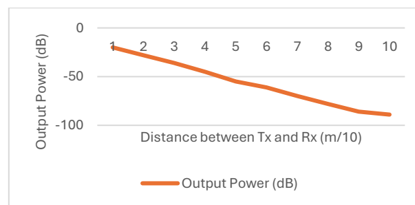
Fig. 14: Output Power for Frequency Doubling Reflectenna System.
