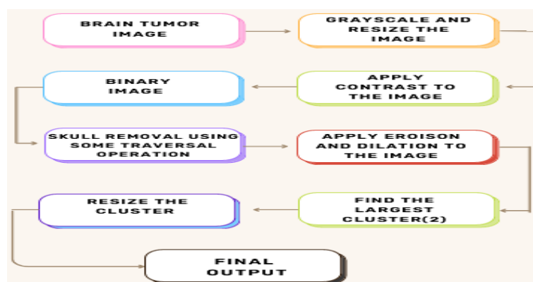
Fig. 2: Tumor Segmentation.
