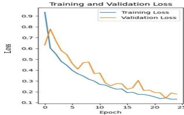
Fig. 6: Training and Validation Loss.
