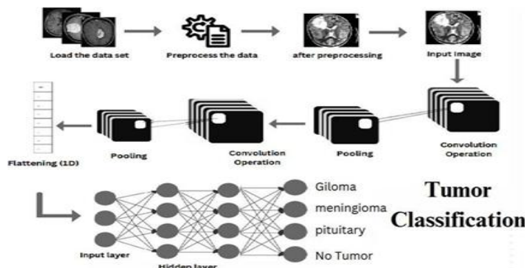
Fig. 1: CNN Architecture for Tumor Classification.
