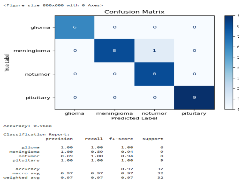
Fig. 7: Confusion Matrix.
