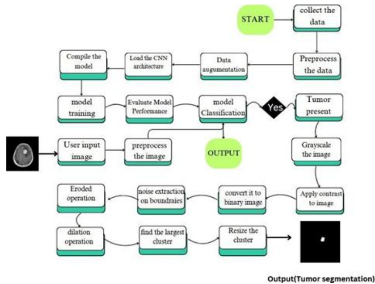
Fig. 4: Proposed Model.
