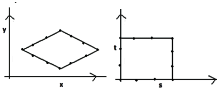
Fig. 1: 12-Noded Rectangular Element Mapped to 12-Noded Standard Square Element
