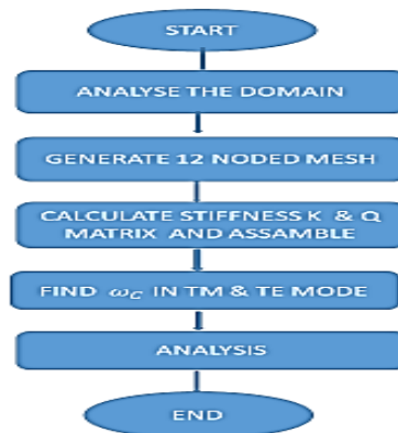
Fig. 3: Flow Chart for Finite Element Process.
