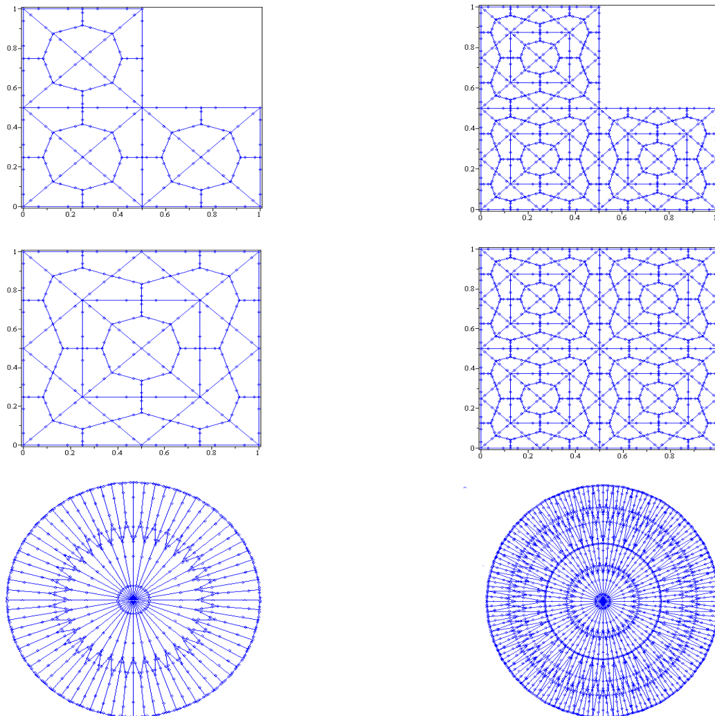
Fig. 2: L, Square and Circular Wave Guide Discretized Into 12-Noded Quadrilateral Meshes.
