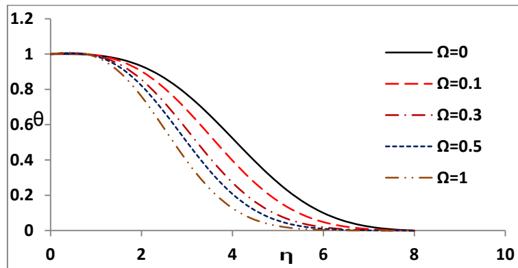
Fig. 5(d) Temperature profiles at \beta_e=5 , \beta_i=0.4 , \Delta=4.5 and M=0.3
