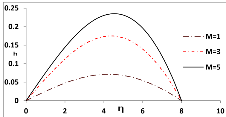
Fig. 4(b) Velocity profiles across the plate at \beta_e=5 , \beta_i=0.4 , \Delta=4.5 and \Omega=0.5
