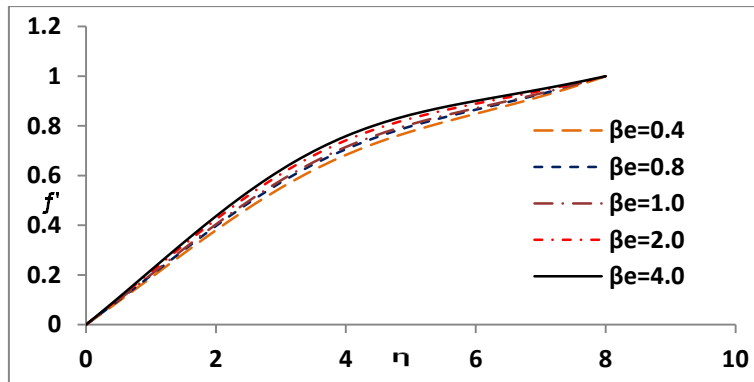
Fig. 1 (a) Velocity profiles along the plate at \beta_i=0.4, \Delta=4.5, M=0.3 and \Omega=0.5
