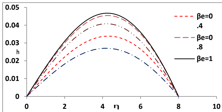
Fig. 1 (b) Velocity profiles across the plate at \beta_i=0.4, \Delta=4.5, M=0.3 and \Omega=0.5
