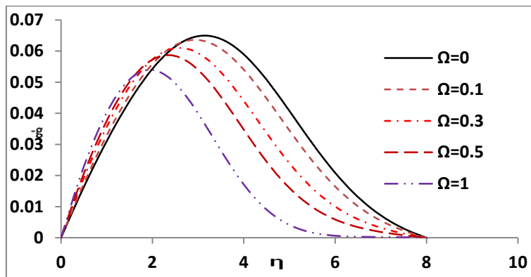
Fig. 5(c) Angular velocity profiles at \beta_e=5, \beta_i=0.4, \Delta=4.5 and M=0.3
