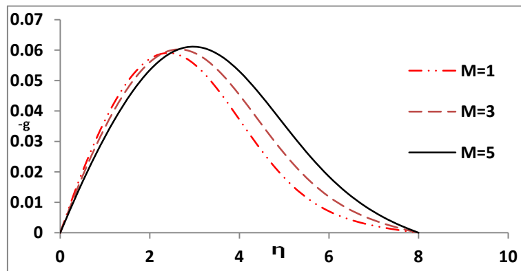
Fig. 4(c) Angular velocity profiles at \beta_e=5 , \beta_i=0.4 , \Delta=4.5 and \Omega=0.5
