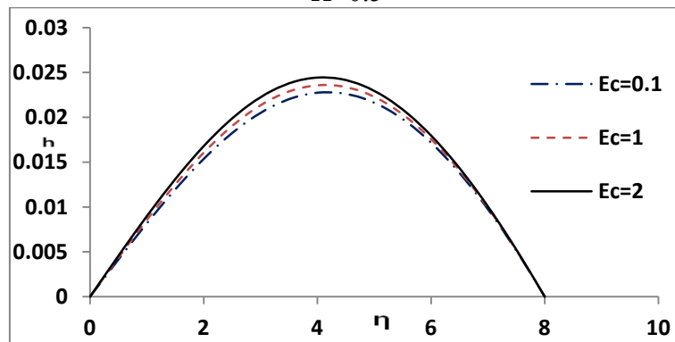
Fig. 6(b) Velocity profiles across the plate at \beta_e=5 , \beta_i=0.4 , \Delta=4.5 and M=0.3, \Omega=0.5
