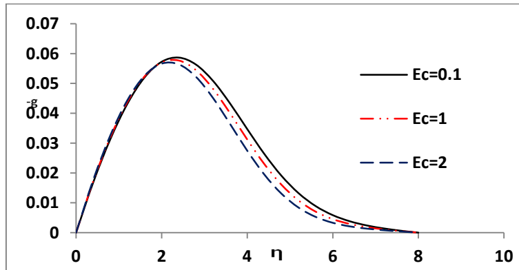
Fig. 6(c) Angular velocity profiles at \beta_e=5, \beta_i=0.4, \Delta=4.5 and M=0.3, \Omega=0.5
