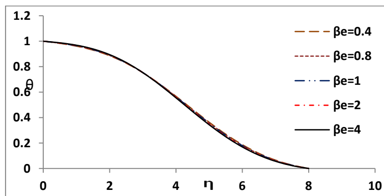
Fig. 1(d) temperature profiles at \beta_i=0.4, \Delta=4.5, M=0.3 and \Omega=0.5
