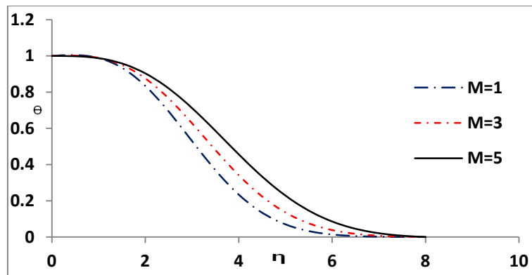
Fig. 4(d) Temperature profiles at \beta_e=5 , \beta_i=0.4 , \Delta=4.5 and \Omega=0.5
