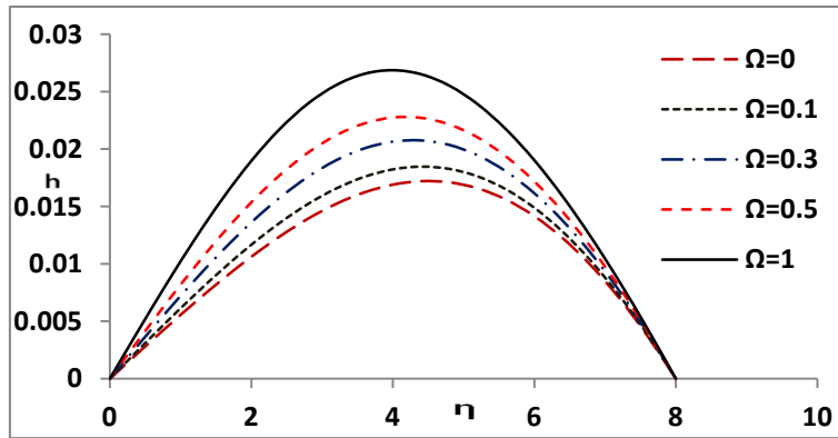
Fig. 5(b) Velocity profiles across the plate at \beta_e=5, \beta_i=0.4, \Delta=4.5 and M=0.3
