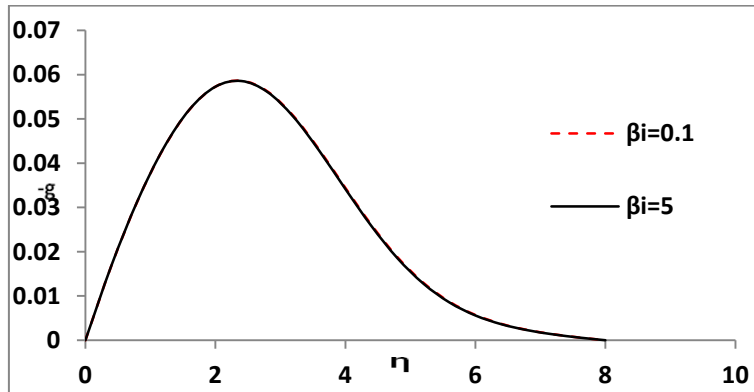
Fig. 2(c) Angular velocity profiles at \beta_e=5, \Delta=4.5, M=0.3 and \Omega=0.5
