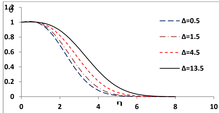
Fig. 3(d) Temperature profiles at \beta_e=5 , \beta_i=0.4 , M=0.3 and \Omega=0.5
