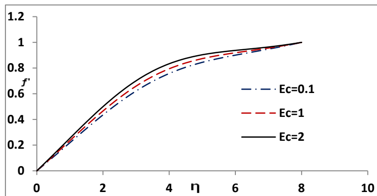
Fig. 6(a) Velocity profiles along the plate at \beta_e=5 , \beta_i=0.4 , \Delta=4.5 and M=0.3 , \Omega=0.5
