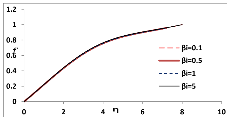
Fig. 2(a) Velocity profiles along the plate at \beta_e=5, \Delta=4.5, M=0.3 and \Omega=0.5
