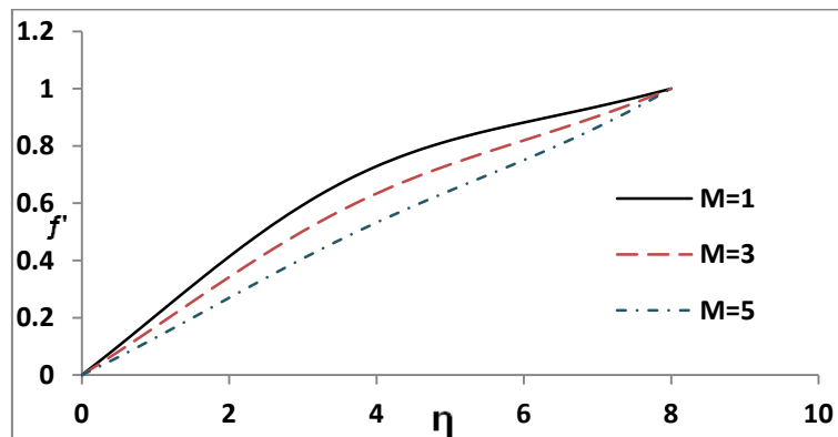
Fig. 4(a) Velocity profiles along the plate at \beta_e=5 , \beta_i=0.4 , \Delta=4.5 and \Omega=0.5
