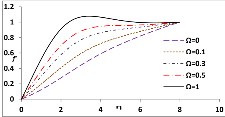
Fig. 5(a) Velocity profiles at \beta_e=5, \beta_i=0.4, \Delta=4.5 and M=0.3
