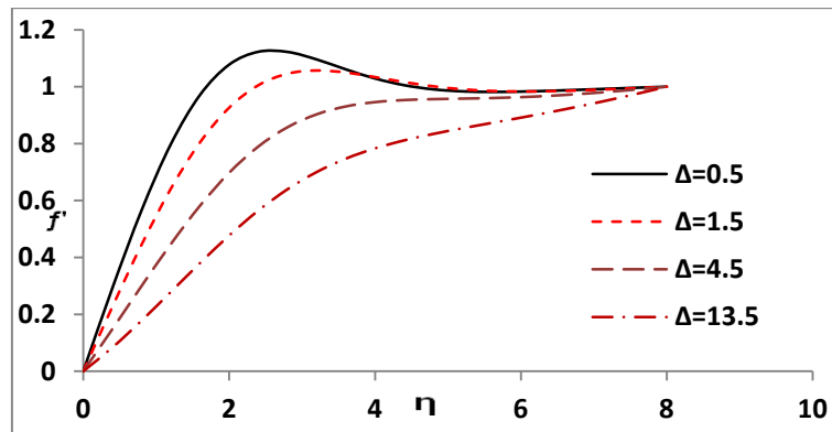
Fig. 3(a) Velocity profiles along the plate at \beta_e=5 , \beta_i=0.4 , M=0.3 and \Omega=0.5
