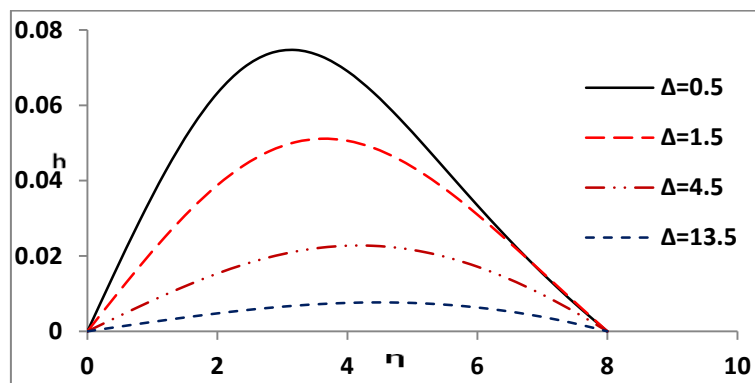
Fig. 3(b) Velocity profiles across the plate at \beta_e=5 , \beta_i=0.4 , M=0.3 and \Omega=0.5
