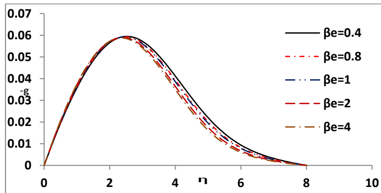
Fig. 1(c) Angular velocity profiles at the plate at \beta_i=0.4, \Delta=4.5, M=0.3 and \Omega=0.5
