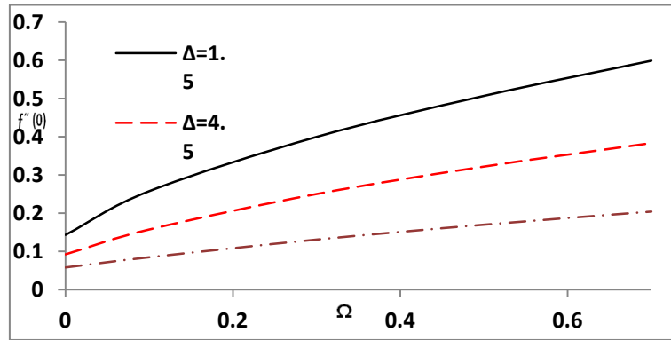
Fig. 7(a) Dimensionless wall shear stress f''(0) as a function of the buoyancy parameter \Omega for various material parameter \Delta ( \beta_e=5 , \beta_i=0.4 and M=0.3 )
