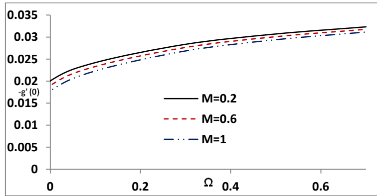
Fig. 8(b) Dimensionless wall couple stress -g'(0) as a function of the buoyancy parameter \Omega for various magnetic parameter M ( \beta_e=5, \beta_i=0.4 and \Delta=4.5 )
