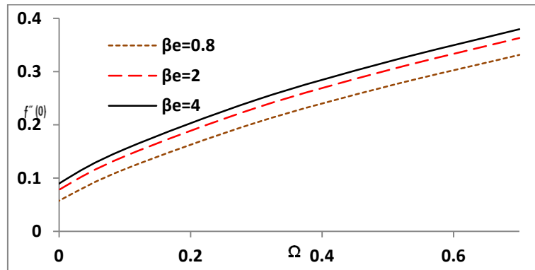
Fig. 9(a) Dimensionless wall shear stress f''(0) as a function of the buoyancy parameter \Omega for various Hall parameter \beta_e ( \beta_i=0.4, \Delta=4.5 and M=0.3 )
