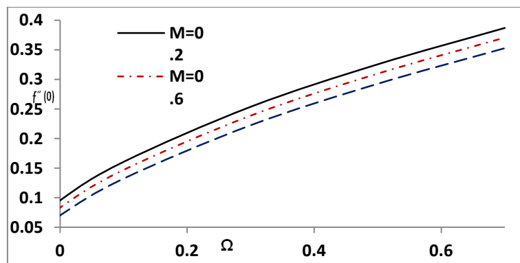
Fig. 8(a) Dimensionless wall shear stress f''(0) as a function of the buoyancy parameter \Omega for various magnetic parameter M ( \beta_e=5 , \beta_i=0.4 and \Delta=4.5 )
