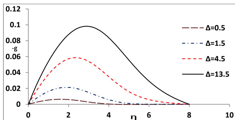
Fig. 3(c) Angular velocity profiles at \beta_e=5 , \beta_i=0.4 , M=0.3 and \Omega=0.5
