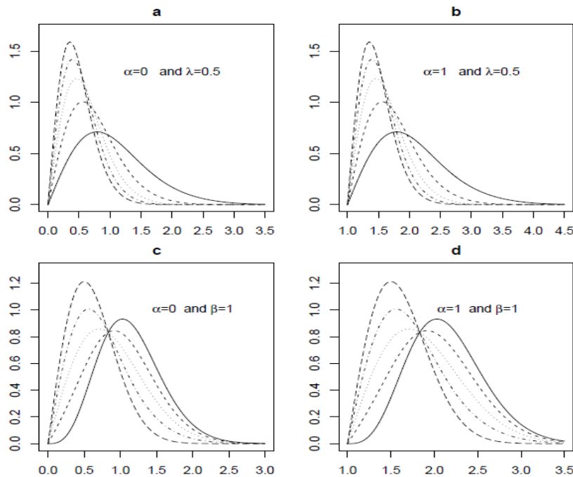
Fig. 2: The pdf's of Various Transmuted two parameters Rayleigh distribution for values of parameters: a) \beta = 0.5[0.5]2.5 , b) \beta = 0.5[0.5]2.5 , c) \lambda = -1[0.5]1 , d) \lambda = -1[0.5]1 with Solid, Dashed, Dotted, Dotdash and Longdash lines respectively.
