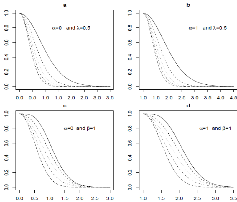
Fig. 3: The reliability function of various Transmuted two parameters Rayleigh distribution for values of parameters: a) \beta = 0.5[0.5]2.5 , b) \beta = 0.5[0.5]2.5 , c) \lambda = -1[0.5]1 , d) \lambda = -1[0.5]1 with Solid, Dashed, Dotted, Dotdash and Longdash Lines Respectively.
