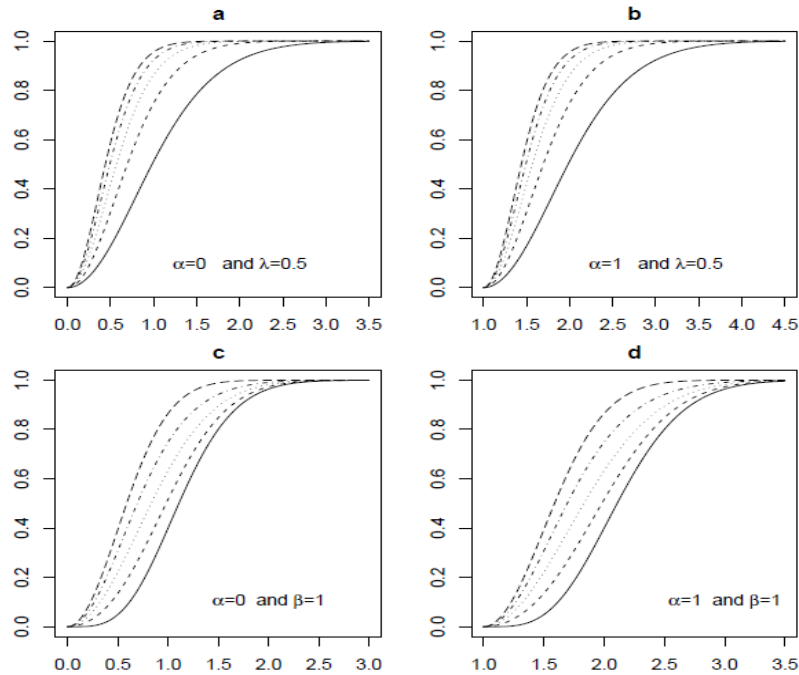
Fig. 1: The cdf's of various Transmuted two parameters Rayleigh Distribution for values of parameters: a) \beta = 0.5[0.5]2.5 , b) \beta = 0.5[0.5]2.5 , c) \lambda = -1[0.5]1 , D) \lambda = -1[0.5]1 with Solid, Dashed, Dotted, Dotdash and Longdash lines respectively.
