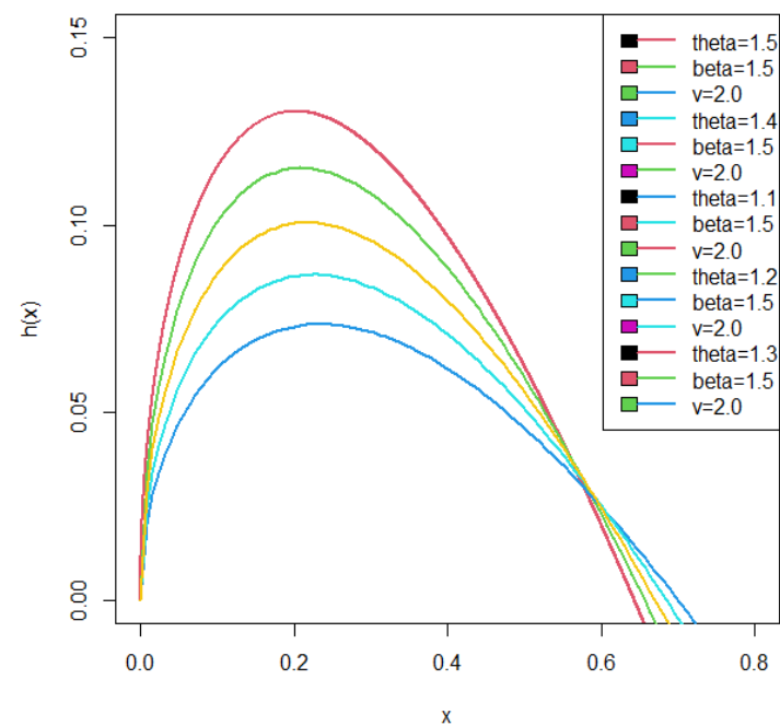
Fig. 4: Hazard Plot of Power Exponentiated Shanker Distribution.
