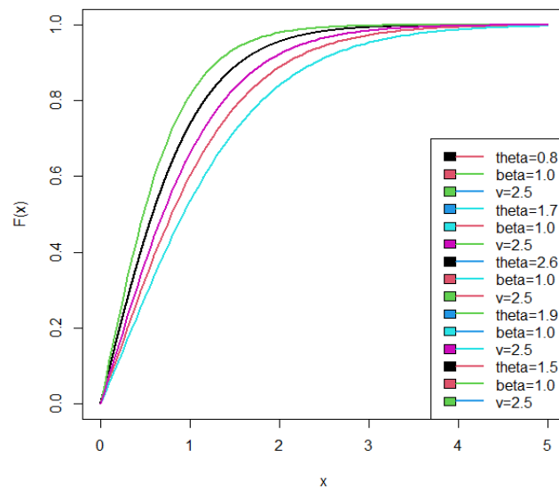
Fig. 2: CDF Plot of Power Exponentiated Shanker Distribution.
