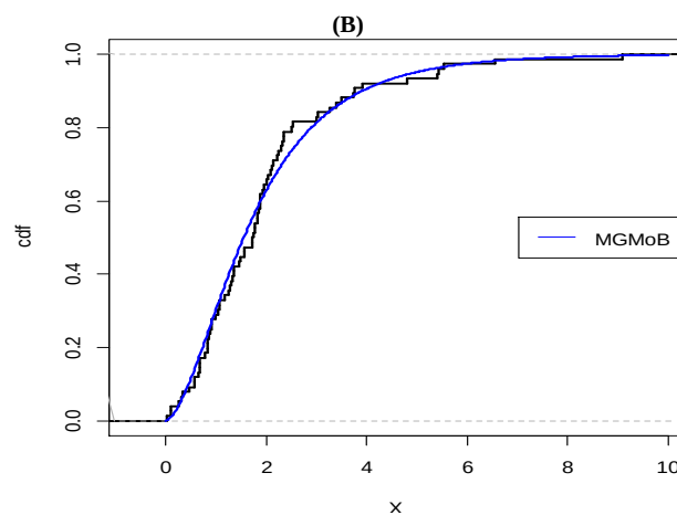
Fig. 3: Plots of Sample and Empirical CDFS of MGMoB Distribution of Data 1A) and 2B).
