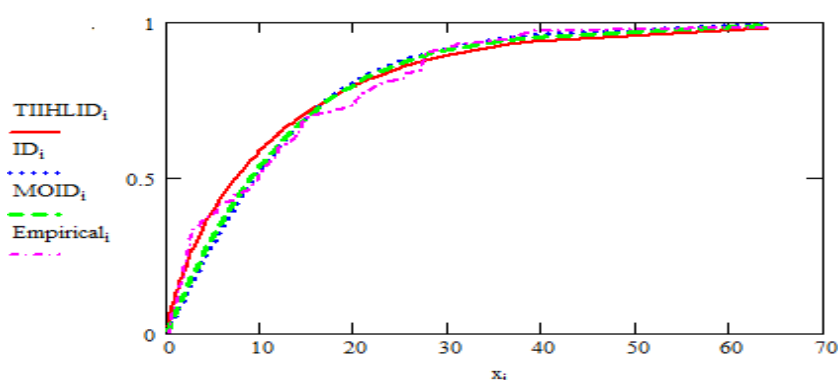
Fig. 4: Empirical, Fitted TIIHLID, ID and M-OID CDF of the Above Data.
