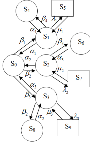
Fig. 2: Transition diagram of Configuration II
