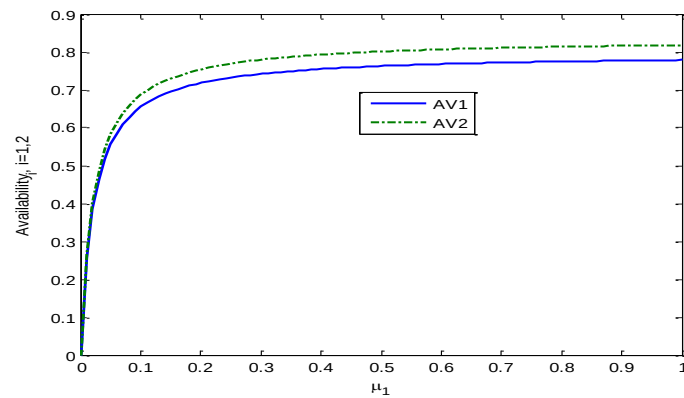
Fig. 9: Availability i versus replacement rate \mu_1
