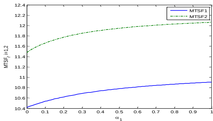
Fig. 5: MTSF_i versus repair rate \alpha_1
