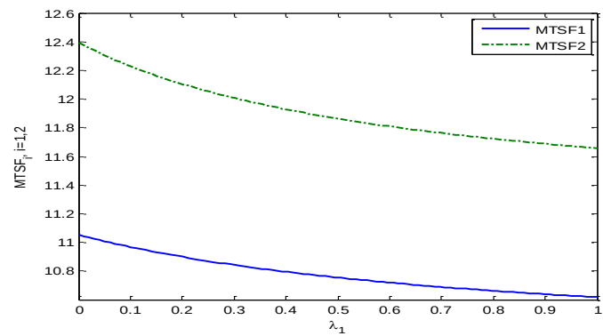
Fig. 3: MTSF_i versus common cause failure \lambda_1
