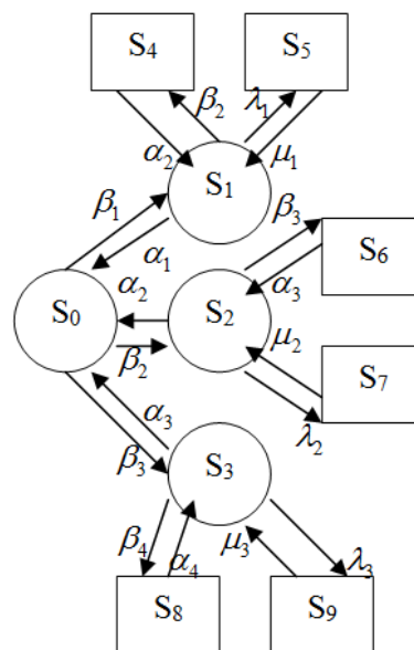
Fig. 1: Transition diagram of Configuration I
