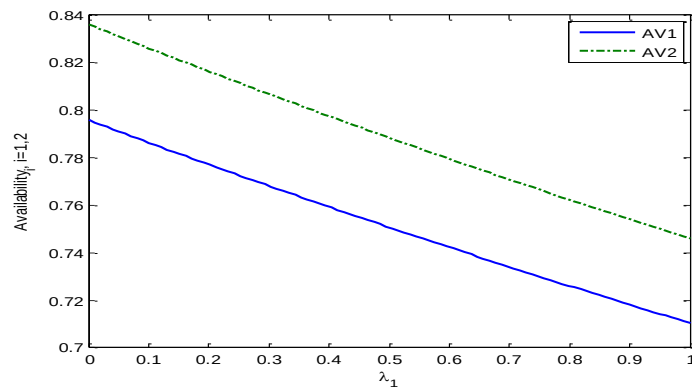
Fig. 8: Availability i versus common cause failure \lambda_1
