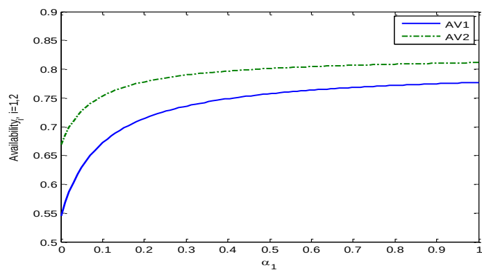
Fig. 6: Availability_i versus repair rate \alpha_1
