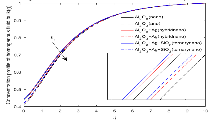
Fig. 5: Variation in Homogenous Fluid Parameter ( K_R ) with the Concentration of Homogenous Bulk Fluid.
