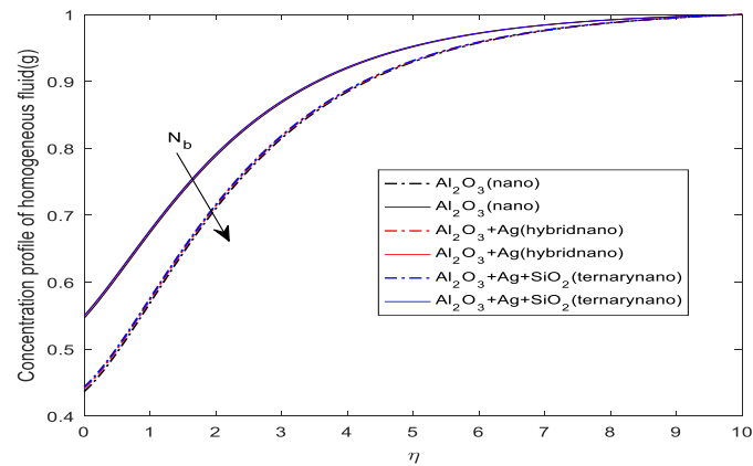
Fig. 8: Variation in Brownian Motion Parameter ( N_B ) with Homogeneous Fluid Concentration.
