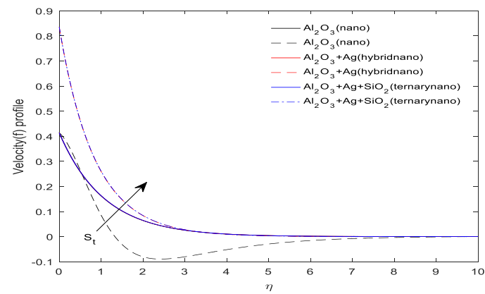
Fig. 4: Variation in Stratification Parameter ( S_T ) with Velocity.
