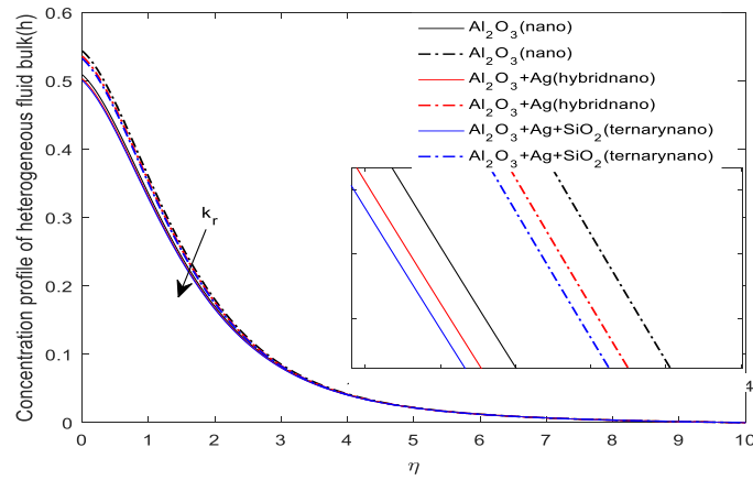
Fig. 6: Variation in Homogenous Parameter ( K_R ) with Reactant B Concentration Profile.
