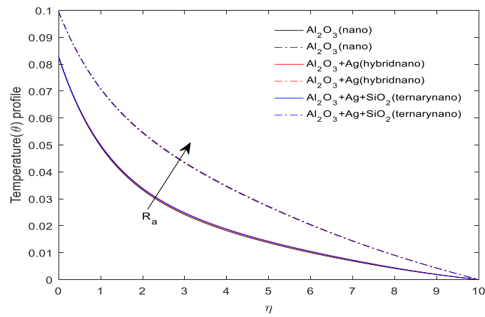
Fig. 2: Variation in Radiation Parameter ( R_A ) with Temperature.
