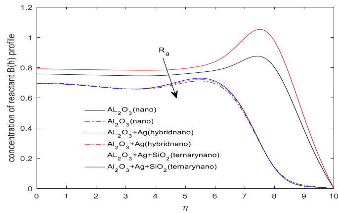
Fig. 3: Variation in Radiation Parameter ( R_A ) with Concentration of Reactant B.
