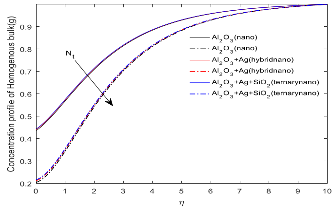
Fig. 7: Variation in Thermophoretic Parameter ( N_T ) with Homogeneous Bulk Concentration Profile.
