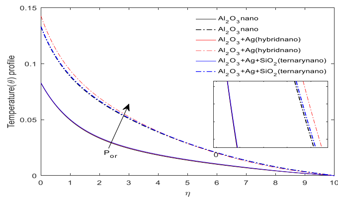
Fig. 1: Variation in Porous Parameter ( P_{or} ) with Temperature.
