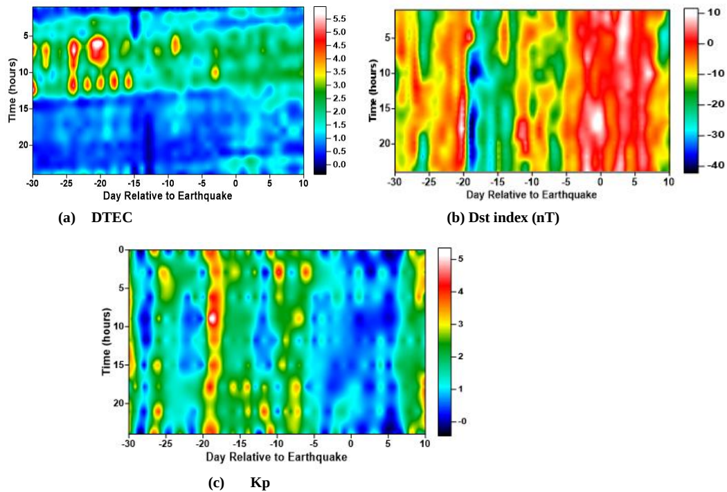
Fig. 2: Results of analysis for the Sichuan earthquake (12 May 2008) from 12 th April to 22 May 2008. The x-axis represents the day relative to the earthquake day. The y-axis represents the time UTC (LT=UTC+08:00). (a) DTEC variations. (b) Variations of Dst geomagnetic index. (c) Variations of Kp geomagnetic index.
