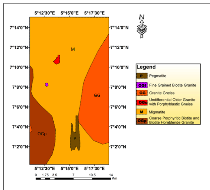
Fig. 2: Geological Map of the Study Area (Akure - Oda - Idanre Area) (Adapted From Nigerian Geological Survey Agency, 2006).
