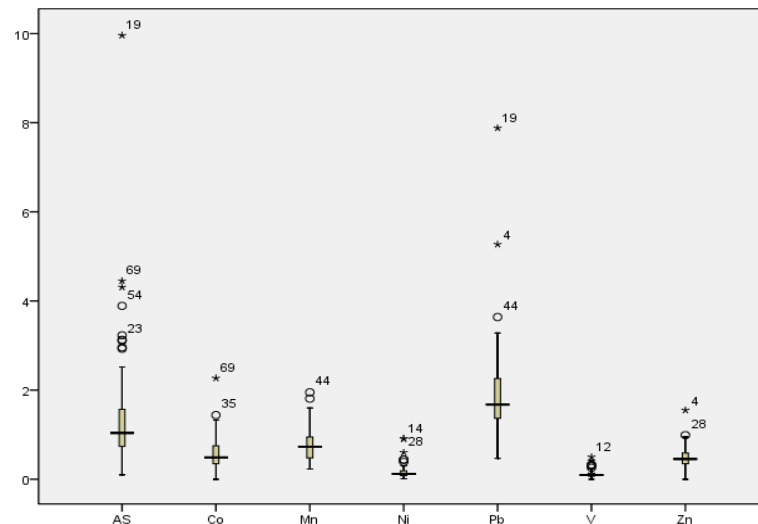
Fig. 5: Box Plots of Enrichment Factors (EF) of the Trace Elements in the Stream Sediments.
