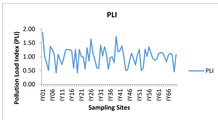
Fig. 7: Pollution Load Index (PLI) Values for Heavy Metals from the Stream Sediment of the Study Area.
