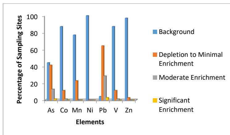
Fig. 6: Percentage Enrichment of Heavy Metals in Stream Sediments from the Study Area.
