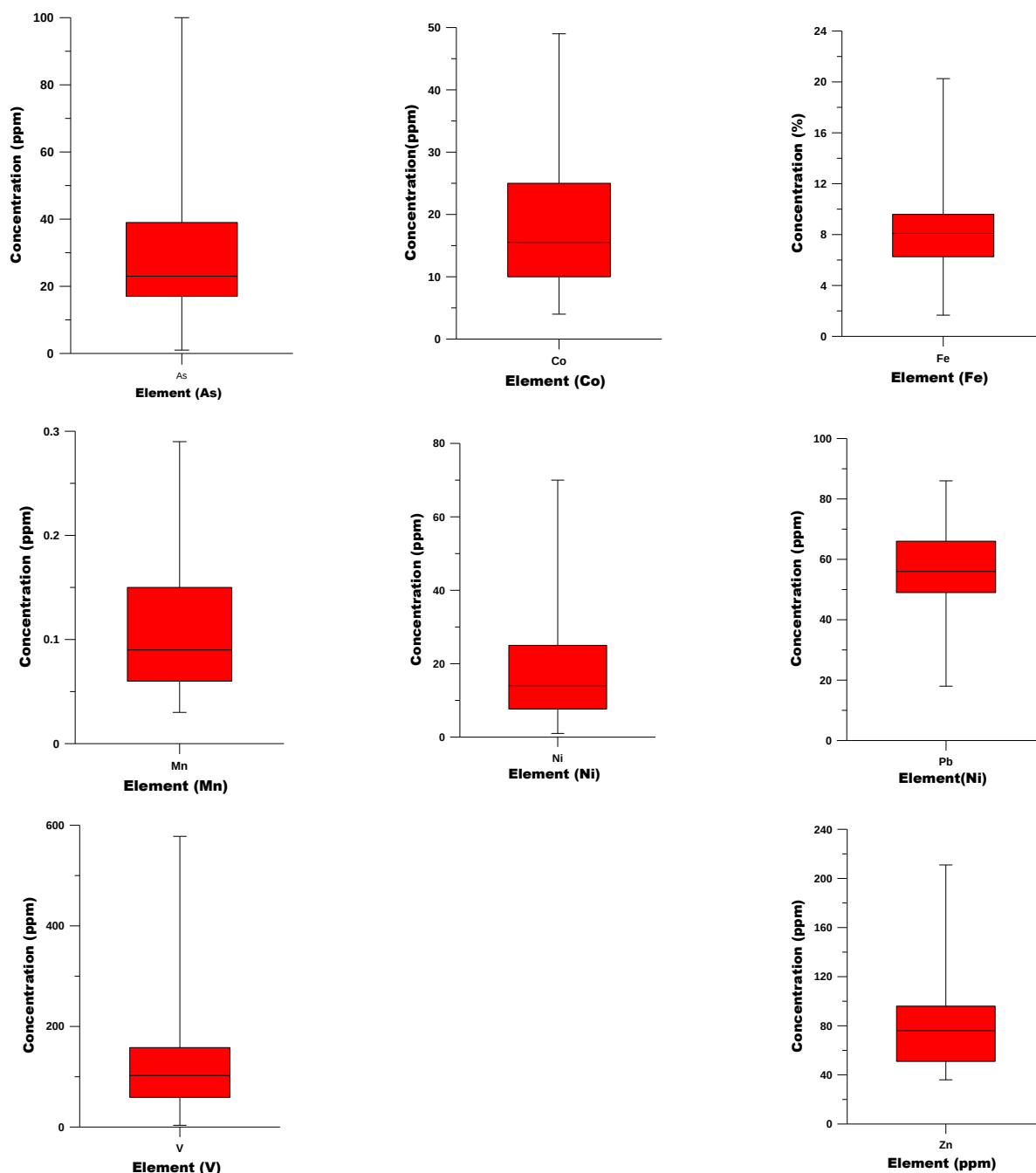
Fig. 4: Box Plot of Trace Element Concentrations in the Stream Sediments from the Study Area.
