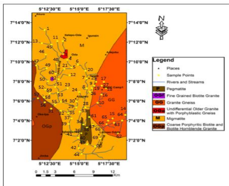
Fig. 3: Geological Map of Akure-Oda-Idanre Area Showing the Sample Locations (Adapted from Nigerian Geological Survey Agency, 2006).
