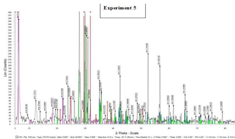
Fig. 12: XRD Analysis of Experiment 5 Containing \text{Fe}^{3+} and Basalt.
