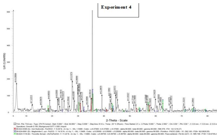
Fig. 11: XRD Analysis of Experiment 4 Containing \text{Fe}^{2+} and Basalt.
