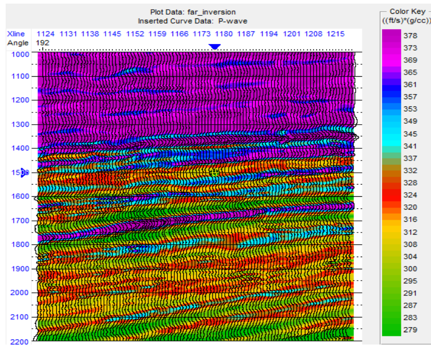
Fig. 12: Model Based Inversion Volume of Far- Angle Stack.
