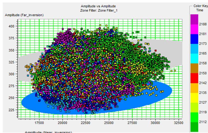
Fig. 13: Crossplot of EI-Near Against EI-Far.
