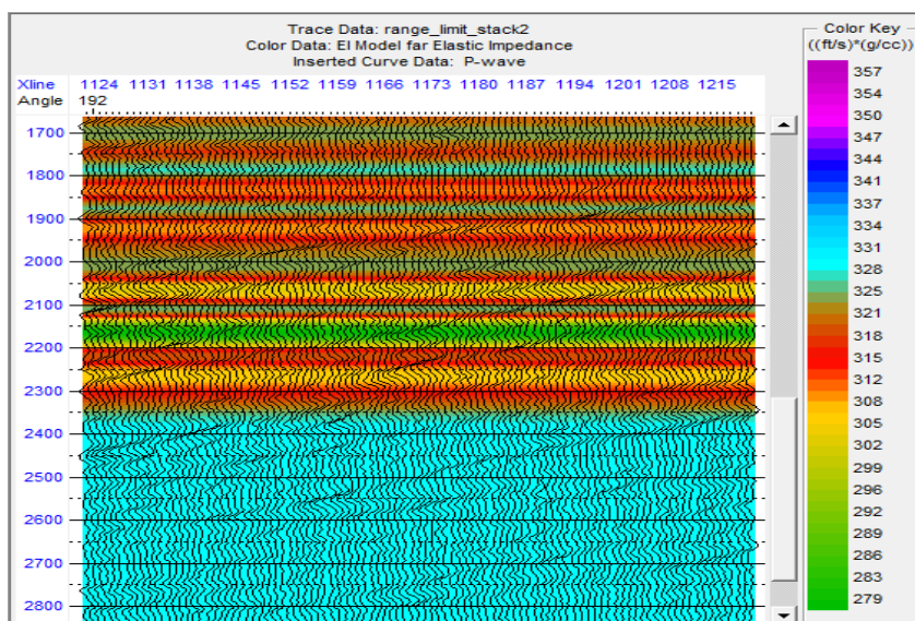
Fig. 10: Elastic Impedance (EI) Far Model Display.
