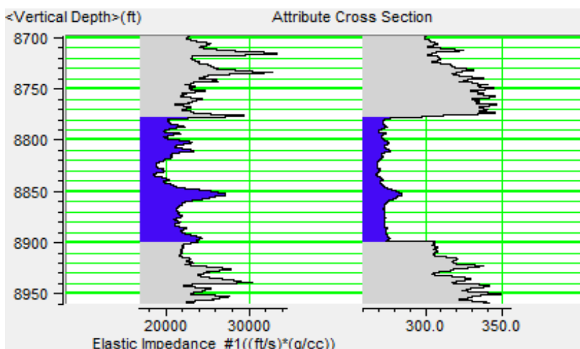
Fig. 5: Attribute Cross Section of the EI Plot.
