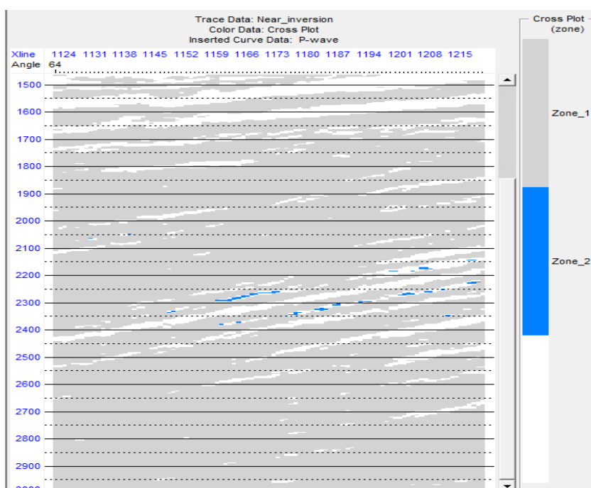
Fig. 15: Near Inversion Volume with Inserted Crossplot. Notice the Changes at the Sand Level which Is Indicative of Gas. That Is, the Elastic Impedance (EI) Is Much Lower on the Far Angle Stack Than the Near Angle Stack.
