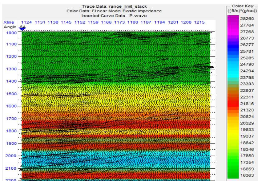
Fig. 9: Elastic Impedance (EI) near Model Display.
