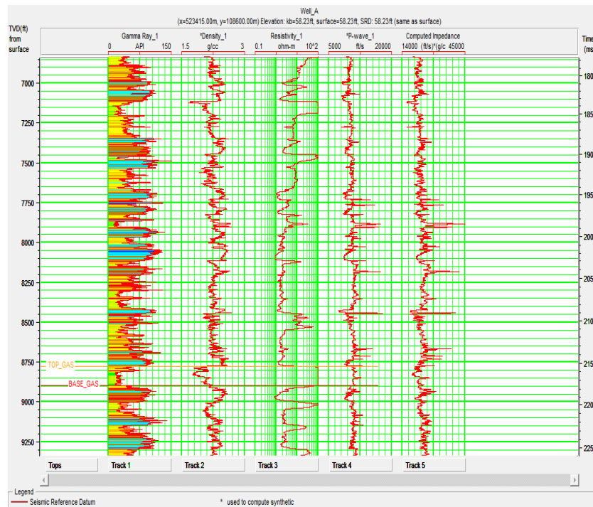
Fig. 2: Wireline Log Data For Well-A Showing Interpreted Mapped Sand Areas.
