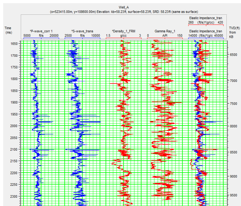
Fig. 3: Modeled Logs After Fluid Substitution.
