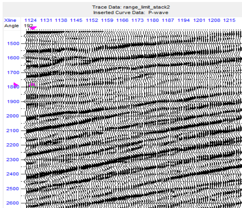
Fig. 8: Range-Limited Far Angle (192m) Stack.
