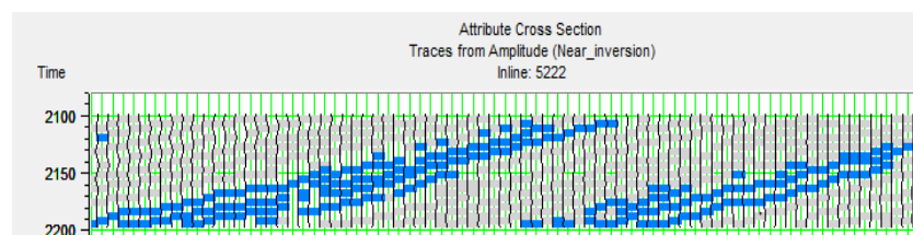
Fig. 14: Attribute Cross Section of the EI Plot with Mapped Zones.
