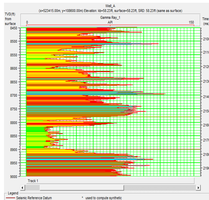
Fig. 1: Close-Up of Gamma Ray Log of Well-A.
