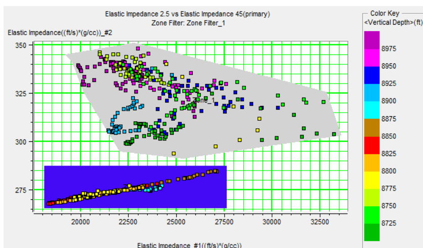
Fig. 4: Crossplot of EI-Near Against EI-Far Showing Mapped Zones.
