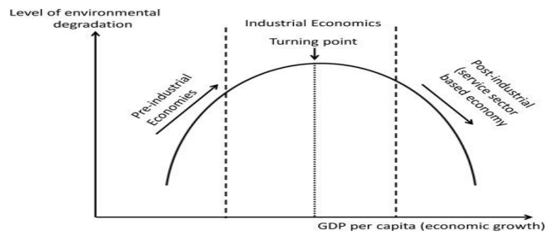
Fig. 3: Environmental Kuznets Curve. Adapted from: Prasad, (2024)
