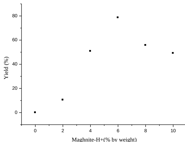
Fig. 8: Effect of the amount of Mag-H + on the yield of the polymerization
