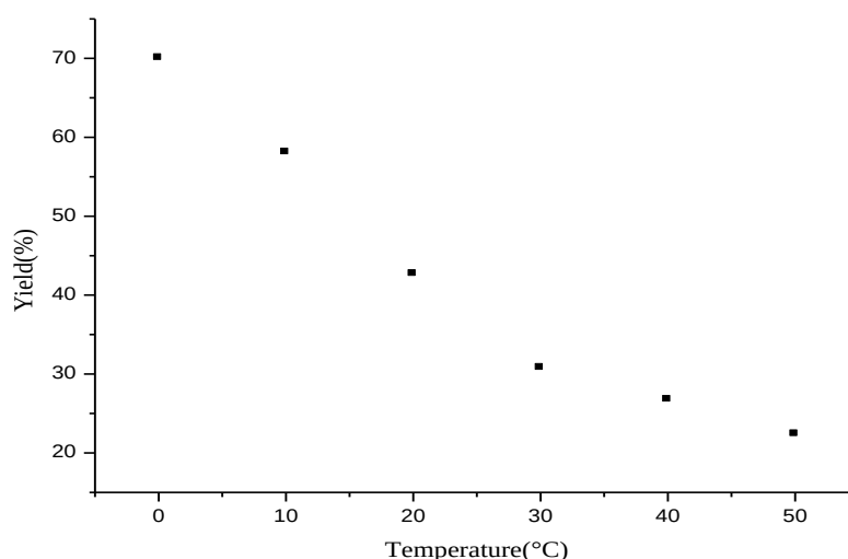
Fig. 9: Effect of the temperature on the yield of polyaniline (Maghnite-H + = 6%, t=3h).
