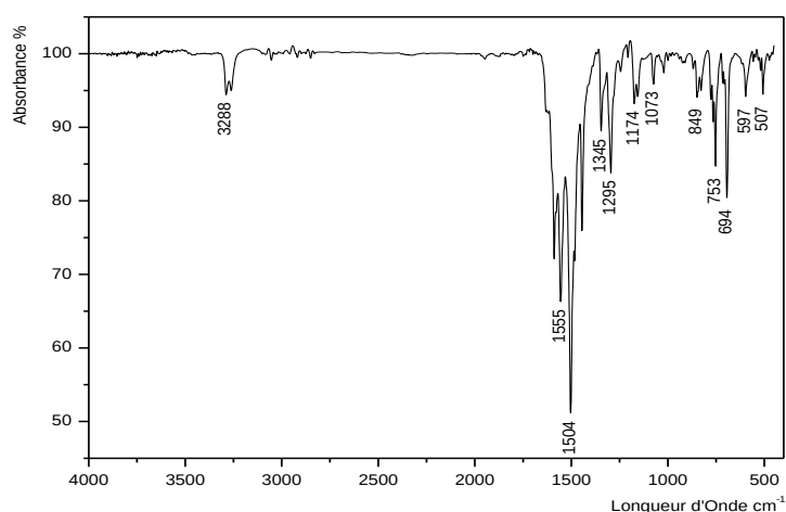
Fig. 1: Shows the characteristic FT-IR spectra of PANI-EB
