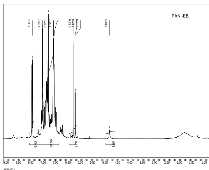
Fig. 4: ^1\text{H} NMR spectrum (300 MHz, \text{CDCl}_3 , Tetramethylsilane (TMS) was used as the internal standard) of polyaniline (PANI-EB) obtained by the polymerization of aniline with \text{Mag-H}^+ initiator system in \text{CDCl}_3 at 25^\circ\text{C} .
