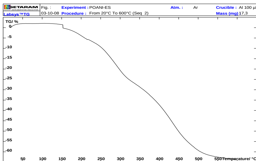
Fig. 7: TGA curves of a pure PANI-ES obtained in nitrogen atmosphere at heating rate of 10 °C/min
