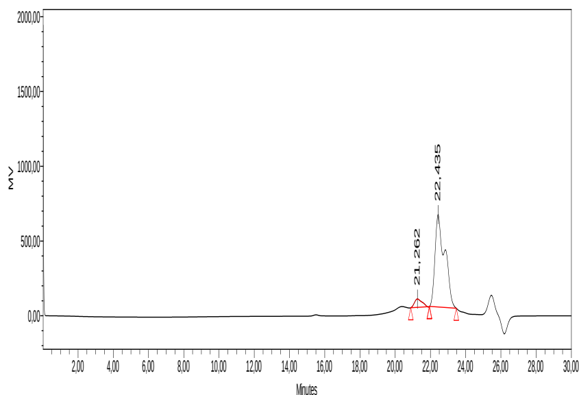
Fig 5: GPC chromatogram of PANI-ES with 6% Mag-H at 0°C for 1 h30 mn ; Number-average molecular weight = 644 g/mol, weight-average molecular weight=746 g/mol, and Polydispersity=1.15.
