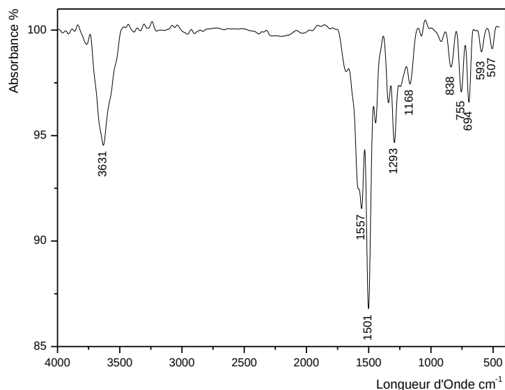
Fig.2: Shows the characteristic FT-IR spectra of PANI-ES
