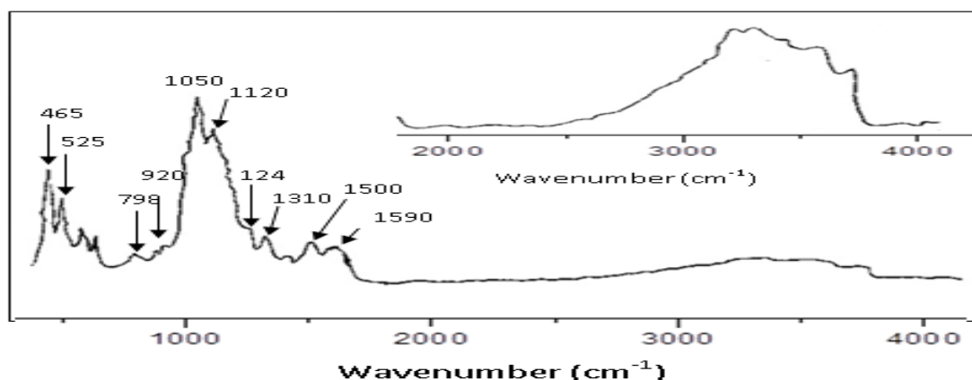
Fig. 5: FT-IR Spectrum for PANI / Ce (III) -MMT.
