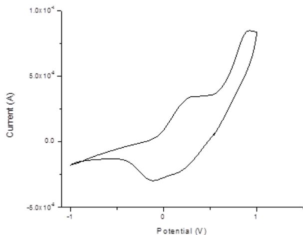
Fig. 9: CV of A PSSA-PANI/Ce (III)-MMT Composite Layer in the Background Electrolyte of 0.1 M KCl. Conditions Used are: Scan Rate of 20 mVs -1 on Pt Working Electrode, Pt-Gauze Counter Electrode, Saturated Calomel Electrode as Reference Electrode
