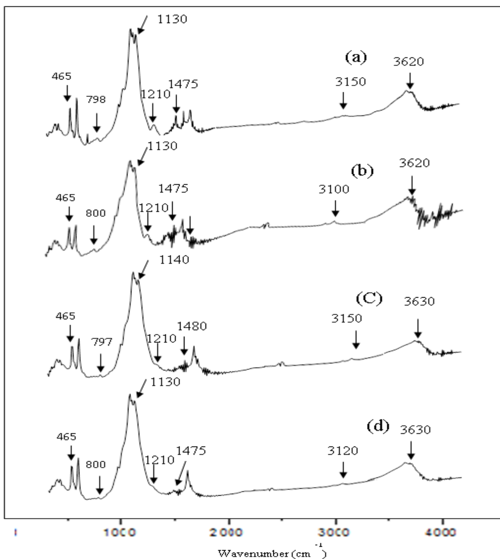
Fig. 6: FT-IR Spectrum for of (A) PSSA-PANI Ce (III)MMT [1:1], (B) PSSA-PANI Ce (III)MMT [1:2], (C) PSSA-PANI Ce (III)MMT [2:3] and (D) PSSA-PANI Ce (III)MMT [3:2].
