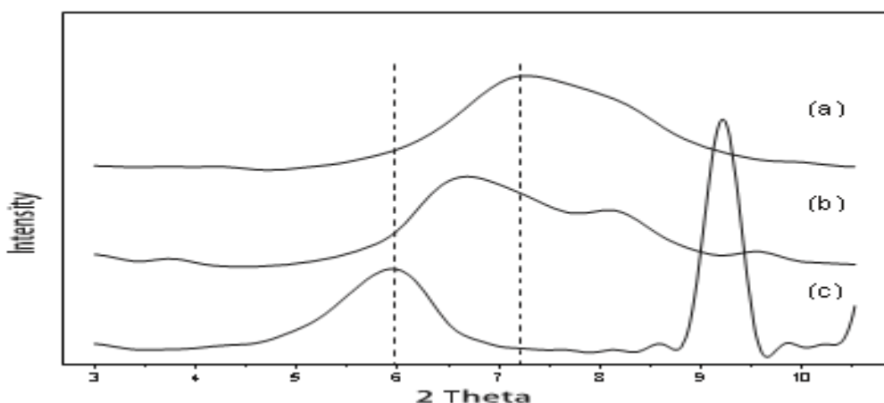
Fig. 2: XRD Patterns of (A) MMT, (B) Ce (IV)-MMT and (C) PANI/ Ce (IV)-MMT.
