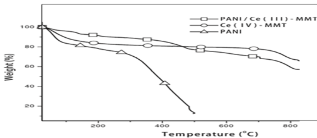
Fig.7: TGA Thermographs for Ce (IV)-MMT, PANI / Ce (III)-MMT, PANI.
