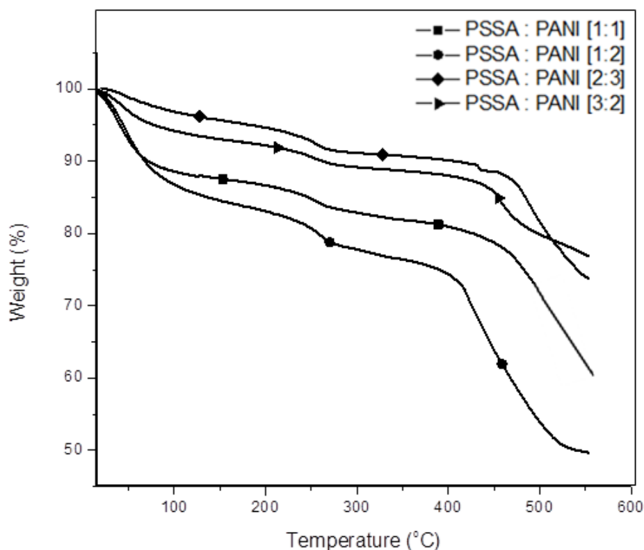
Fig.8: TGA Thermograms of PSSA-PANI /Ce (III)-MMT [1:1], PSSA-PANI /Ce (III)-MMT [1:2], PSSA-PANI /Ce (III)-MMT [2:3], and PSSA-PANI /Ce (III)-MMT [3:2].
