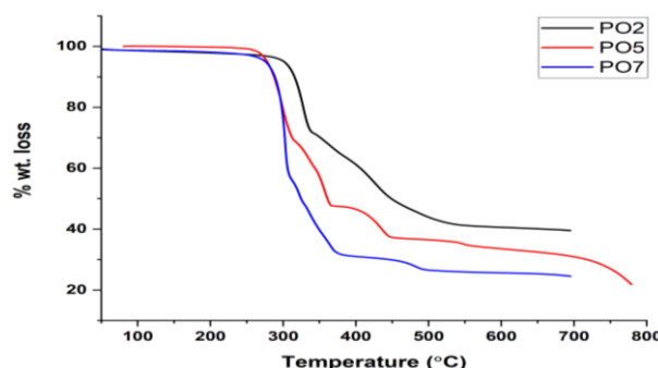
Fig. 2: Thermogravimetric Analysis of Macrocyclic Complexes.
