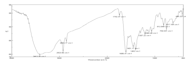
Fig. 4: FT-IR Spectroscopy of Complex
