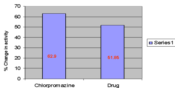
Fig. 12: Comparison of Chlorpromazine with Schiff Base Derivative
