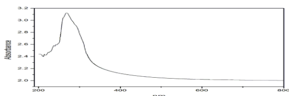
Fig. 1: UV-Visible Spectroscopy of Ligand
