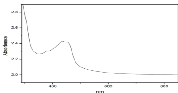
Fig. 2: UV-Visible Spectroscopy of Complex
