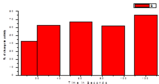
Fig. 11: % of Change in Activity with Time
