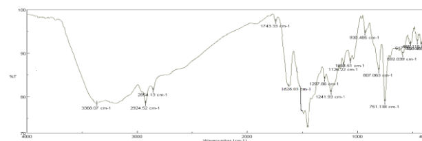
Fig. 3: FT-IR Spectroscopy of Ligand
