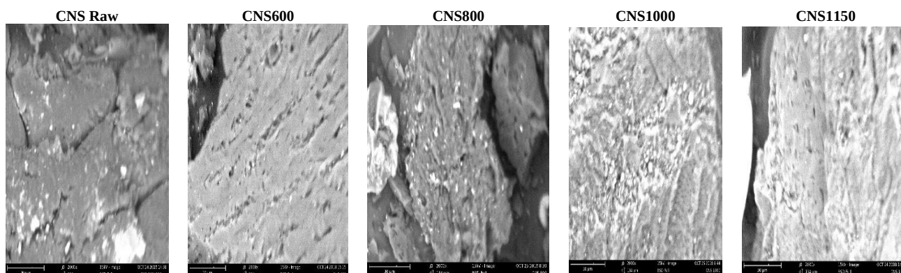
Fig. 5: Scanning Electron Micrograph of Coconut Shell and Its Char Samples.
