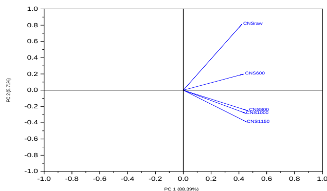
Fig. 4: Loading Plot for CNS Samples.
