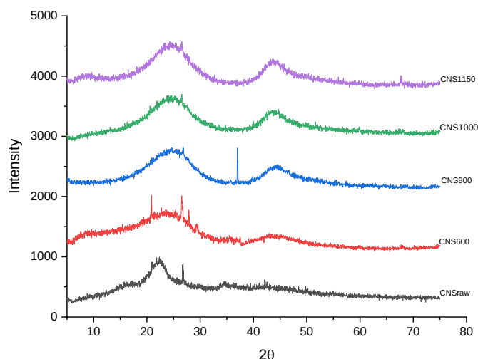
Fig. 3: CNS Raw and Char Samples Diffractograms.
