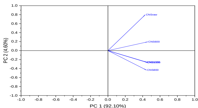
Fig. 2: PCA Loading Plot of Spectra Data.
