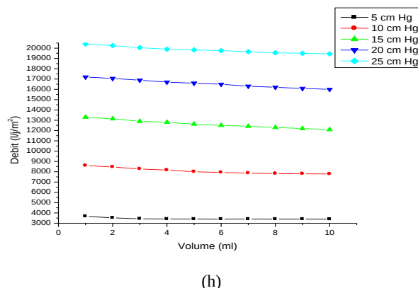
Fig. 4: Evolution of the flow of distilled water depending on the pressure (g) and the volume of filtrate at different pressures (h).
