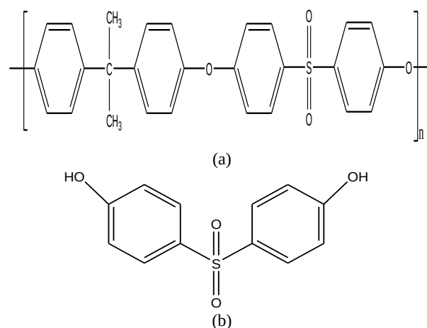
Fig. 1: Chemical structures of polysulfone (PSU) (a) and 4,4-sulfoxydiphenol S (b).
