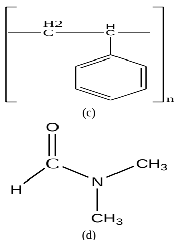
Fig. 2: Chemical structures of expanded polystyrene (c) and N, N-dimethylformamide (d).
