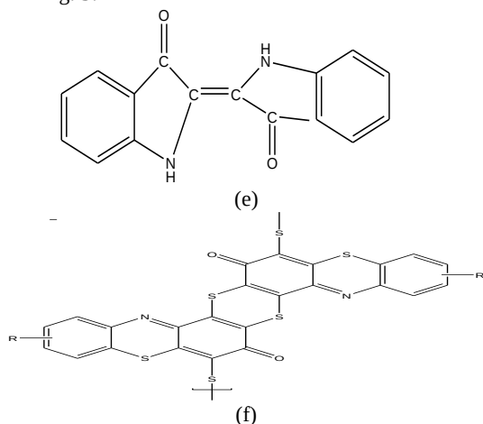
Fig. 3: Chemical structures of vat dyes (Indigo (e) and Black sulphur (f)).
