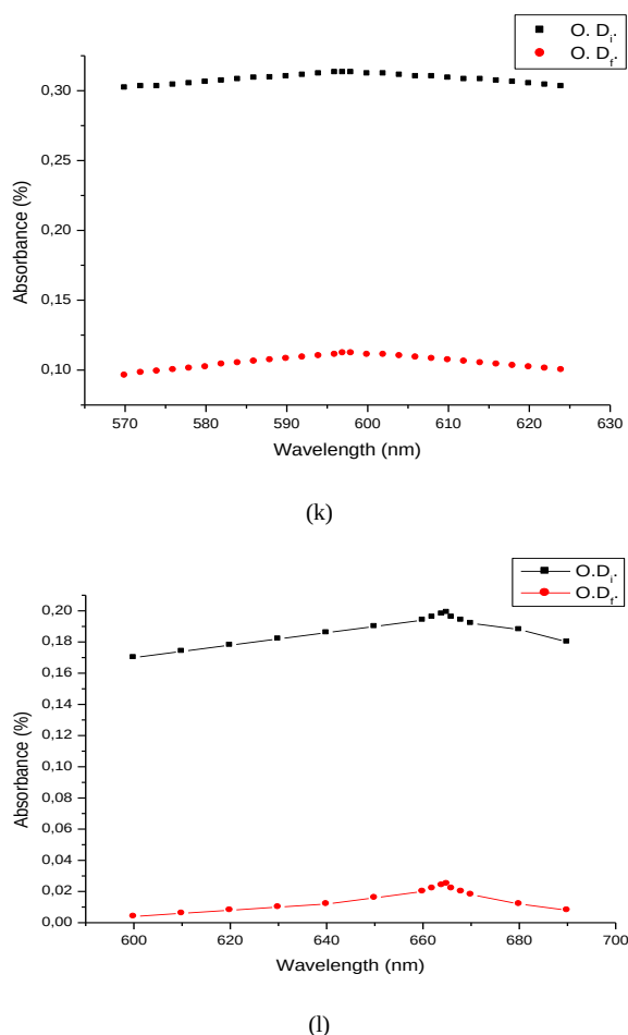
Fig. 10: Curves of absorbance of the effluent collected dyes compounds (black sulphur (k), indigo (l))
