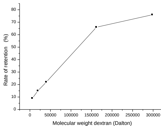
Fig. 5: Evolution of the retention of the membrane as a function of dextran molecular mass
