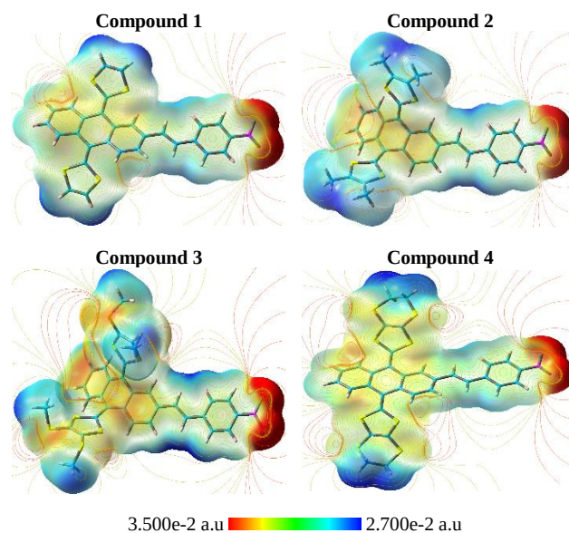
Fig. 2: Molecular Electrostatic Potential Surface of (Extf) Derivatives 1-4.
