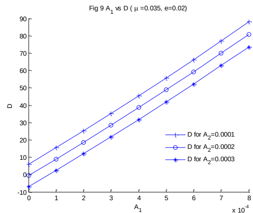
Fig. 9: A1 Vs D for M= 0.035, E=0.02.
