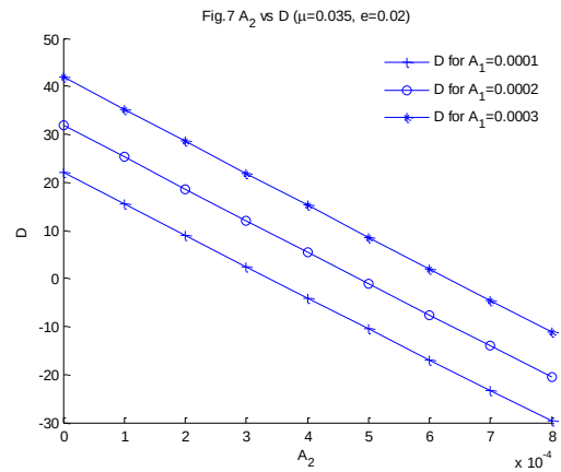
Fig. 7: A2 Vs D for M= 0.035, E=0.02.
