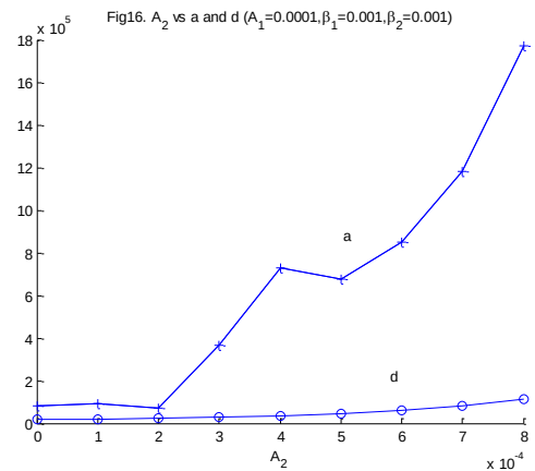
Fig. 16: A2 vs 'a' and 'd' for A1=0.0001, B1=0.001, B2=0.001.
