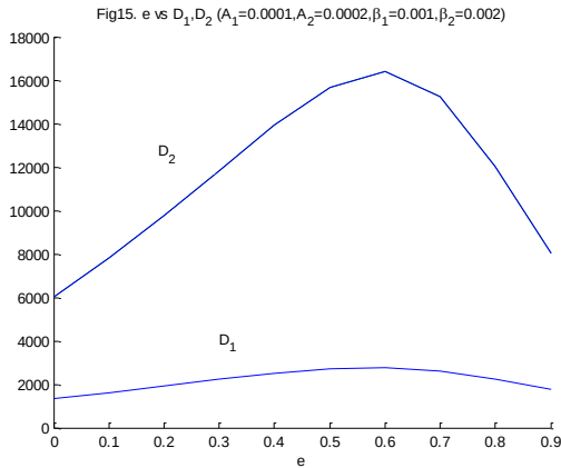
Fig. 15: "e" vs D1, D2 for A1=0.0001, A2=0.0002, B1=0.001, B2=0.002.
