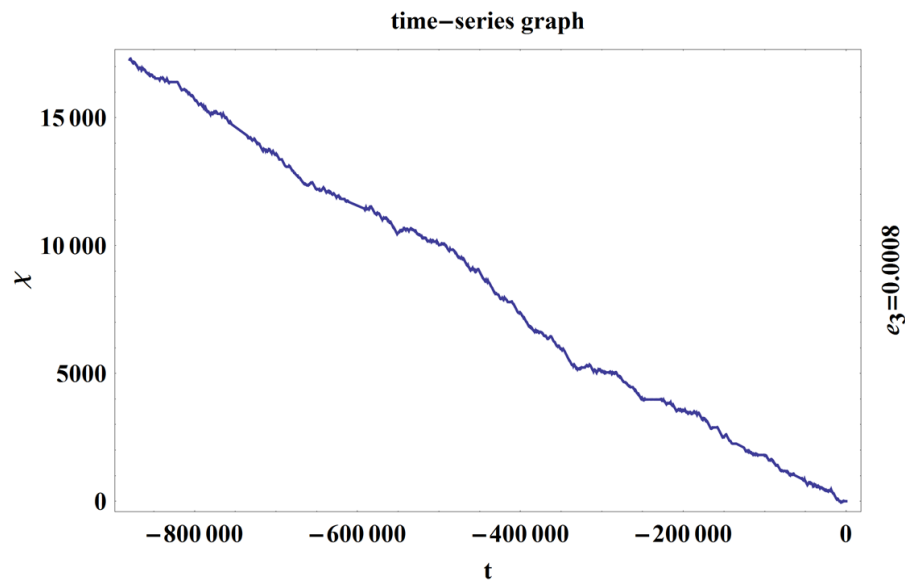
Fig. 4.2: Time-Series Graph at i_3^2, i_1^2 e_3, i_1 i_3 e_3 and i_3^2 e_3 Resonances with Oblateness of Saturn. Secular Resonances of All Inner Satellites Have Been Considered at i_1=1.62^\circ, i_3=1.093^\circ and e_3=0.0008 .
