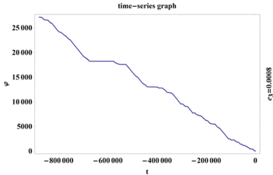
Fig. 4.4: Time-Series Graph at i_1 i_3, i_1^2 e_3, i_1 i_3 e_3 and i_3^2 e_3 Resonances with Oblateness of Saturn. Secular Resonances of All Inner Satellites Have Been Considered at i_1 = 1.62^\circ, i_3 = 1.093^\circ and e_3 = 0.0008 .
