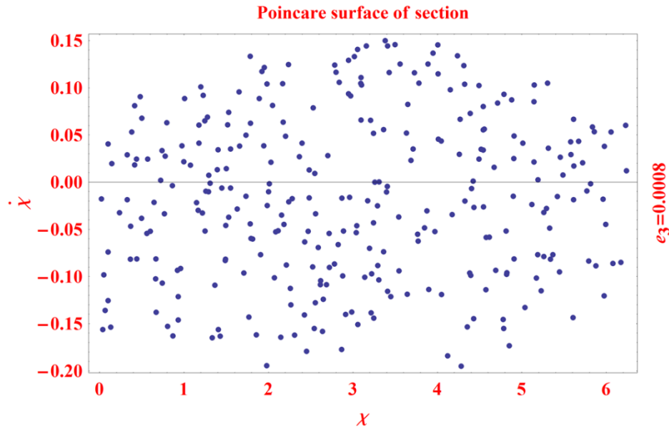
Fig. 4.1: Poincare Surface of Section at i_3^2, i_1^2 e_3, i_1 i_3 e_3 and i_3^2 e_3 Resonances with Oblateness of Saturn. Secular Resonances of All Inner Satellites Have Been Considered at i_1=1.62^\circ, i_3=1.093^\circ and e_3=0.0008 .
