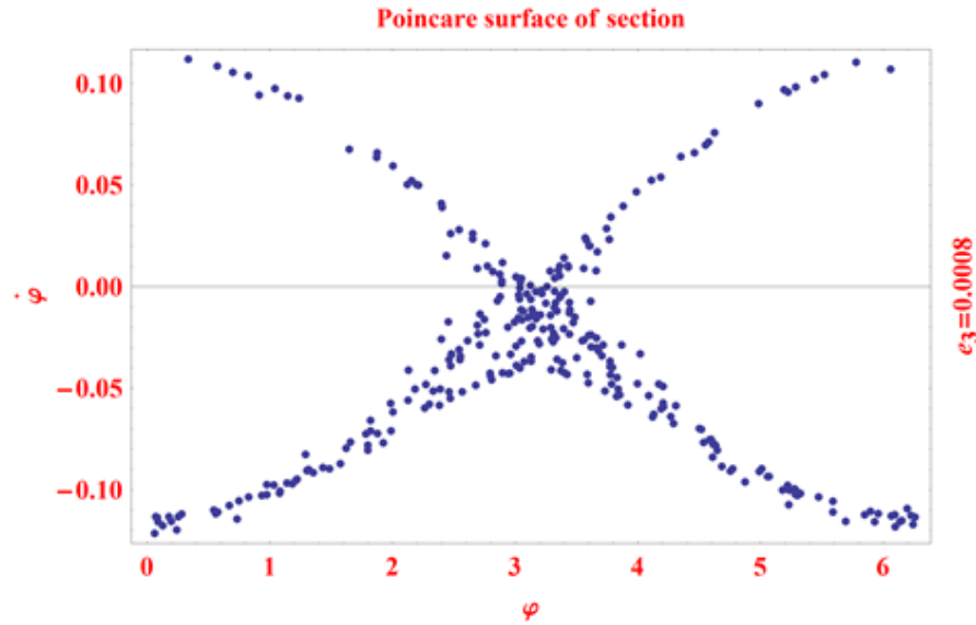
Fig. 4.3: Poincare Surface of Section at i_1 i_3, i_1^2 e_3, i_1 i_3 e_3 and i_3^2 e_3 Resonances with Oblateness of Saturn. Secular Resonances of All Inner Satellites Have Been Considered at i_1 = 1.62^\circ, i_3 = 1.093^\circ and e_3 = 0.0008 .
