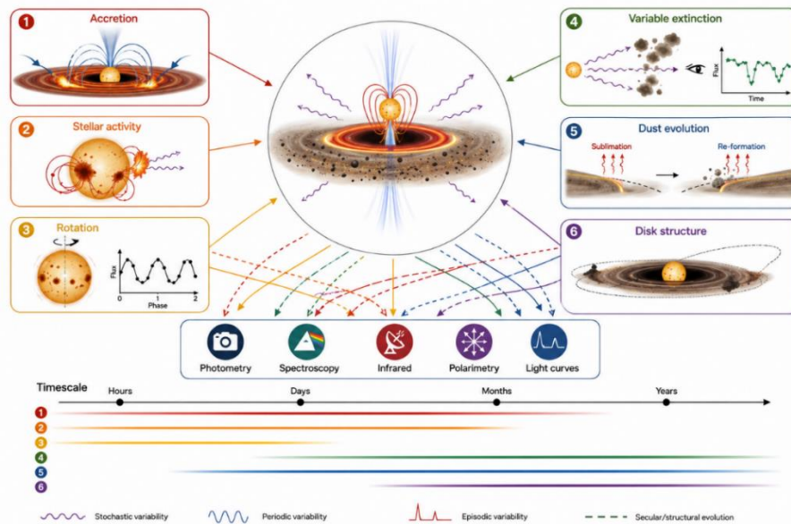
Fig. 2: Major Variability Mechanisms in Young Stellar Systems, Linking Accretion, Stellar, Extinction, Dust, and Circumstellar Structural Processes with Their Characteristic Observational Behaviour.
