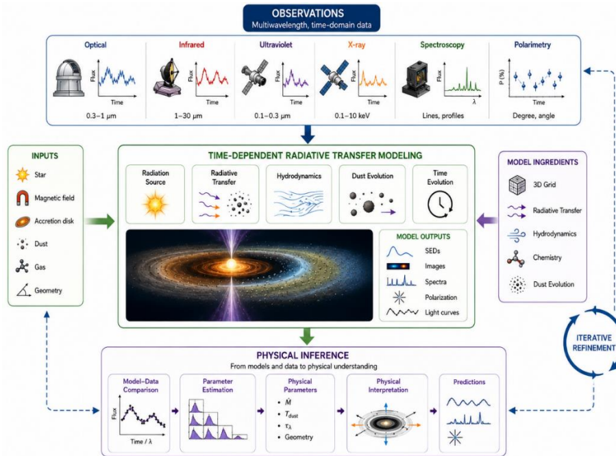
Fig. 5: Future Research Framework Integrating Multiwavelength Time-Domain Observations, Time-Dependent Radiative-Transfer Modelling, and Physical Inference for Evolving Circumstellar Environments.
