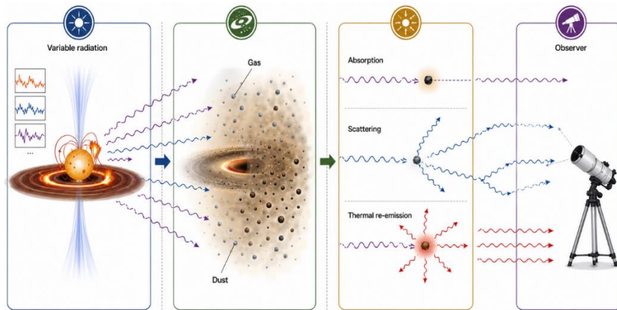
Fig. 1: Schematic Representation of Time-Dependent Radiation–Matter Interaction in A Young Stellar System, Showing Variable Stellar/Accretion Radiation, Circumstellar Dust and Gas, Absorption, Scattering, Thermal Re-Emission, and the Resulting Radiation Received by an Observer.
