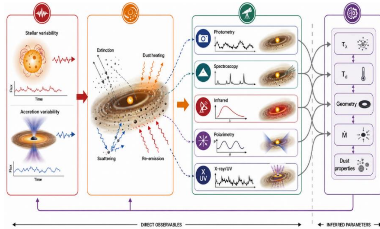
Fig. 3: Connection between Variable Radiation, Circumstellar Response, Observational Diagnostics, and Inferred Physical Parameters in Young Stellar Systems.
