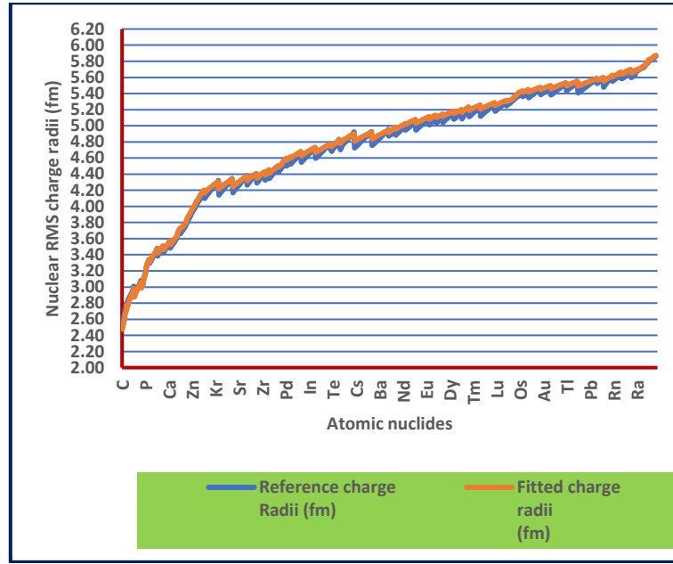
Fig. 1: Fitted Nuclear RMS Charge Radii.
