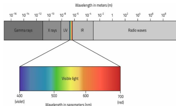
Fig. 3: Electromagnetic Spectrum.
