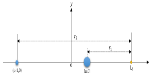
Fig. 3: Location of L_3 in the X-Y Plane.
