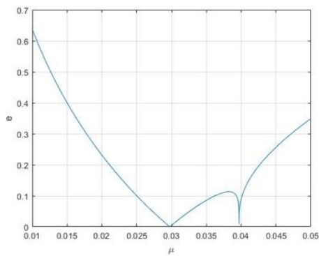
Fig. 7: Transition Curve when A_2 = 0 and \Xi = 0.01
