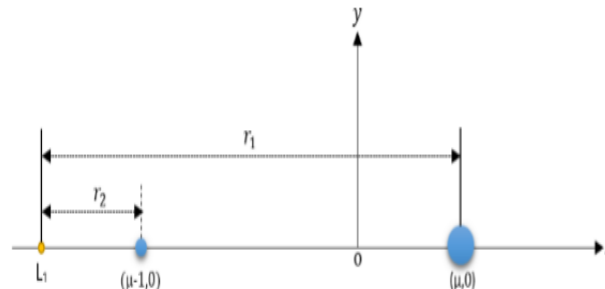
Fig. 1: Location of L_1 in the X-Y Plane.
