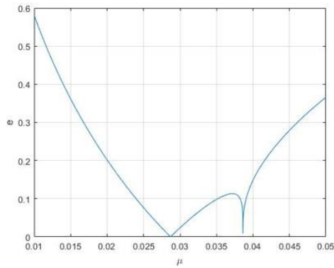
Fig. 5: Transition Curve When A_2 = 0.003 and \xi = 0.001
