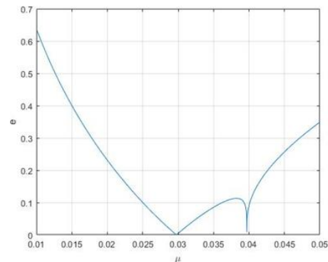
Fig. 7: Transition Curve when A_2 = 0 and \Xi = 0.01
