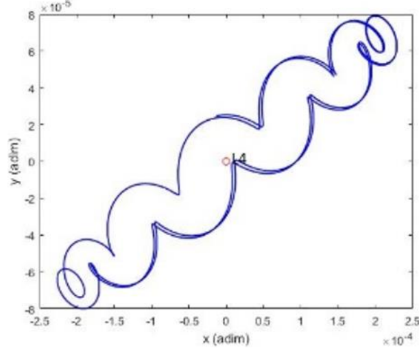
Fig. 10: Tadpole Orbit Around L_4 Point for Sun-Jupiter in A Rotating-Pulsating Coordinate System.
