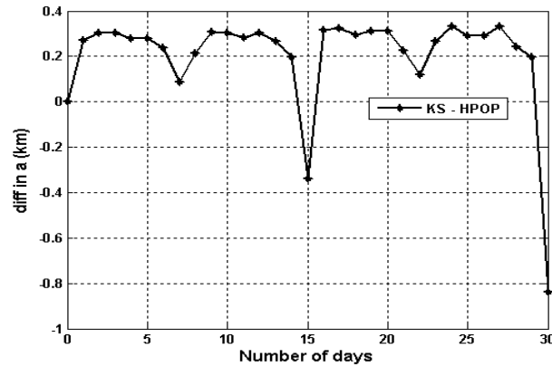
Fig. 10: Difference between KS and HPOP in Semi-Major Axis.
