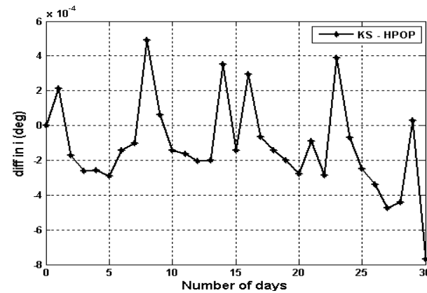
Fig. 12: Difference between KS and HPOP in Inclination.
