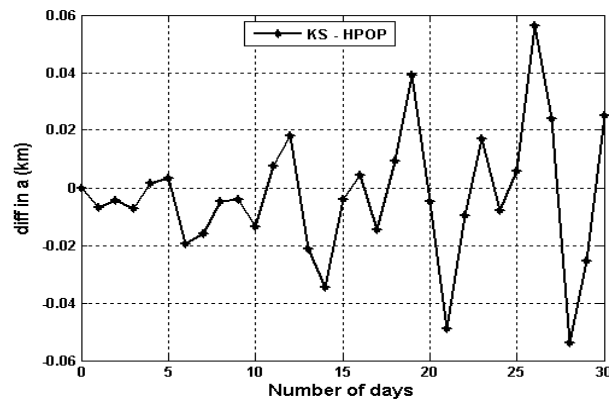
Fig. 1: Difference Between KS and HPOP in Semi-Major Axis.
