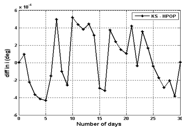
Fig. 9: Difference between KS and HPOP in Inclination.
