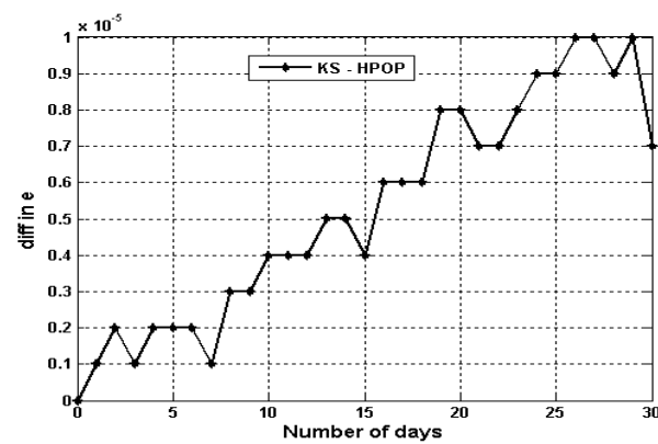
Fig. 8: Difference Between KS and HPOP in Eccentricity.
