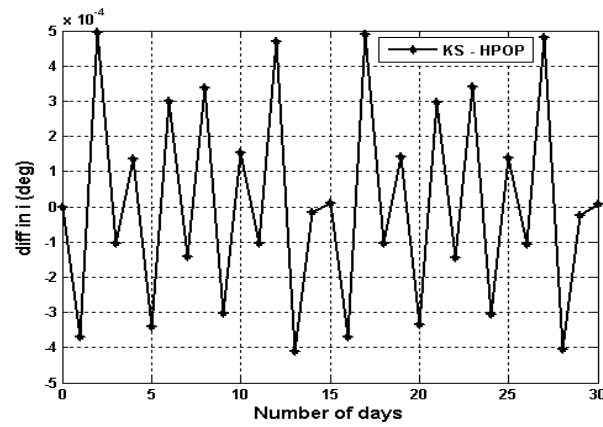
Fig. 3: Difference Between KS and HPOP in Inclination.
