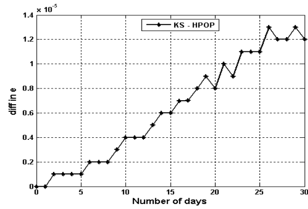
Fig. 2: Difference Between KS and HPOP in Eccentricity.
