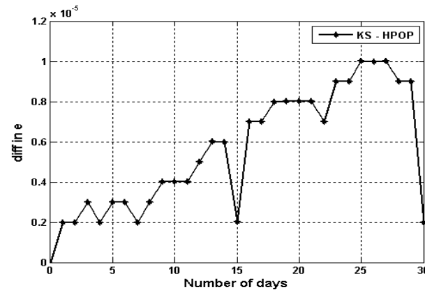
Fig. 11: Difference between KS and HPOP in Eccentricity.
