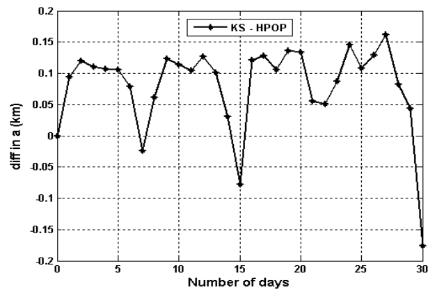
Fig. 7: Difference Between KS and HPOP in Semi-Major Axis.
