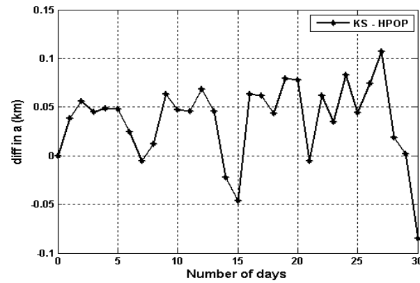
Fig. 4: Difference Between KS and HPOP in Semi-Major Axis.
