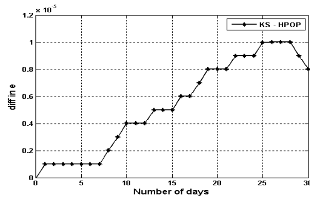
Fig. 5: Difference between KS and HPOP in Eccentricity.
