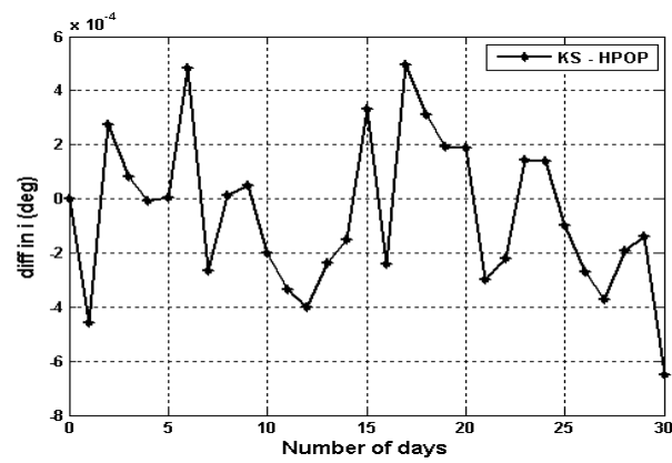
Fig. 6: Difference between KS and HPOP in Inclination.
